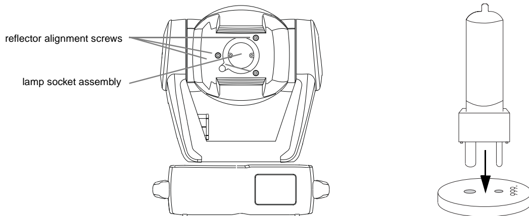
Figure 1: Lamp installation
