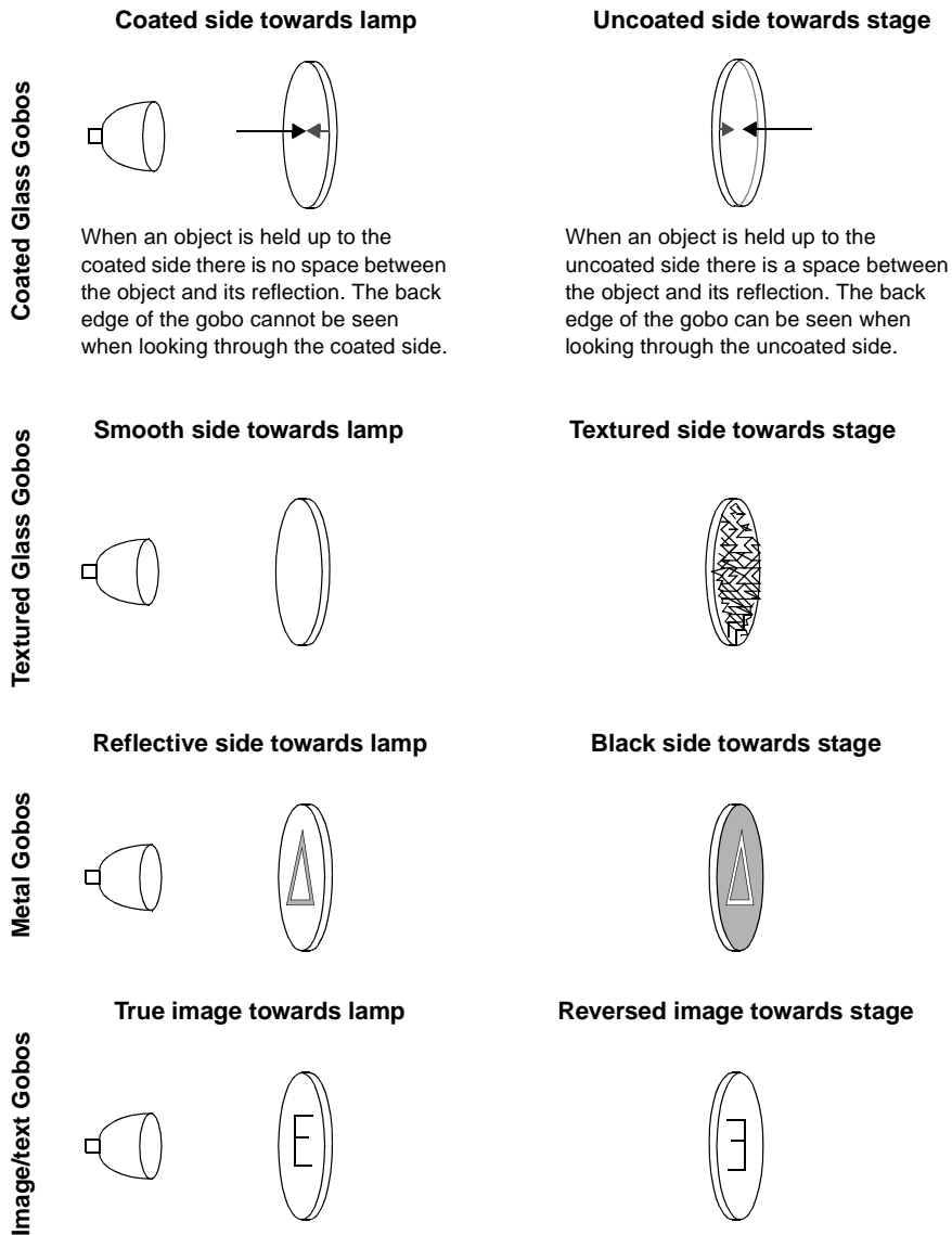
Figure 7: Gobo orientation
