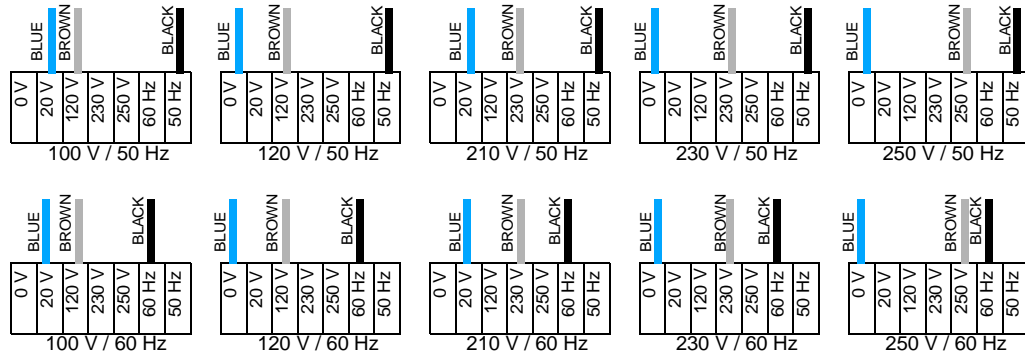
Figure 12: Voltage and frequency settings
