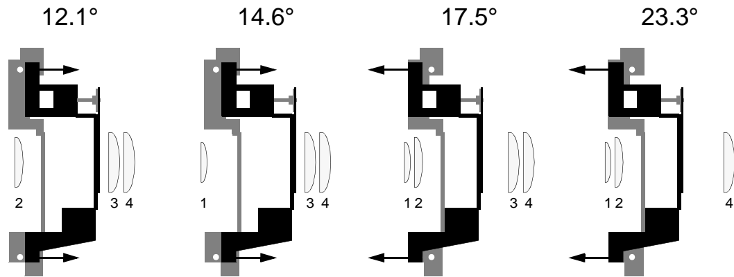
Figure 9: MAC 250 optical configurations
