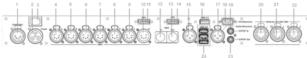
grandMA3 full-size rear panel
