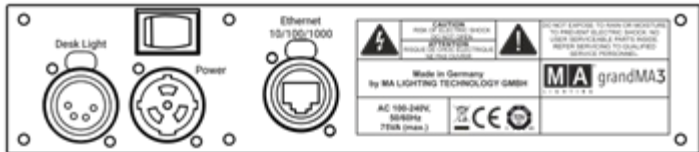
grandMA3 extension – rear panel
